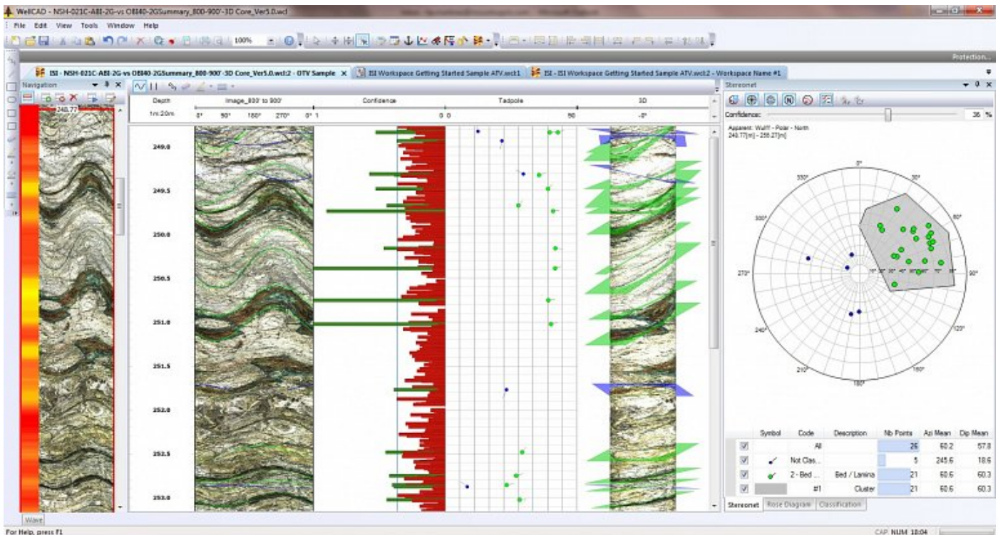
The Image & Structure Interpretation (ISI) module for WellCAD provides a comprehensive tool kit for analysing image logs. Image courtesy of Mount Sopris Instruments.
