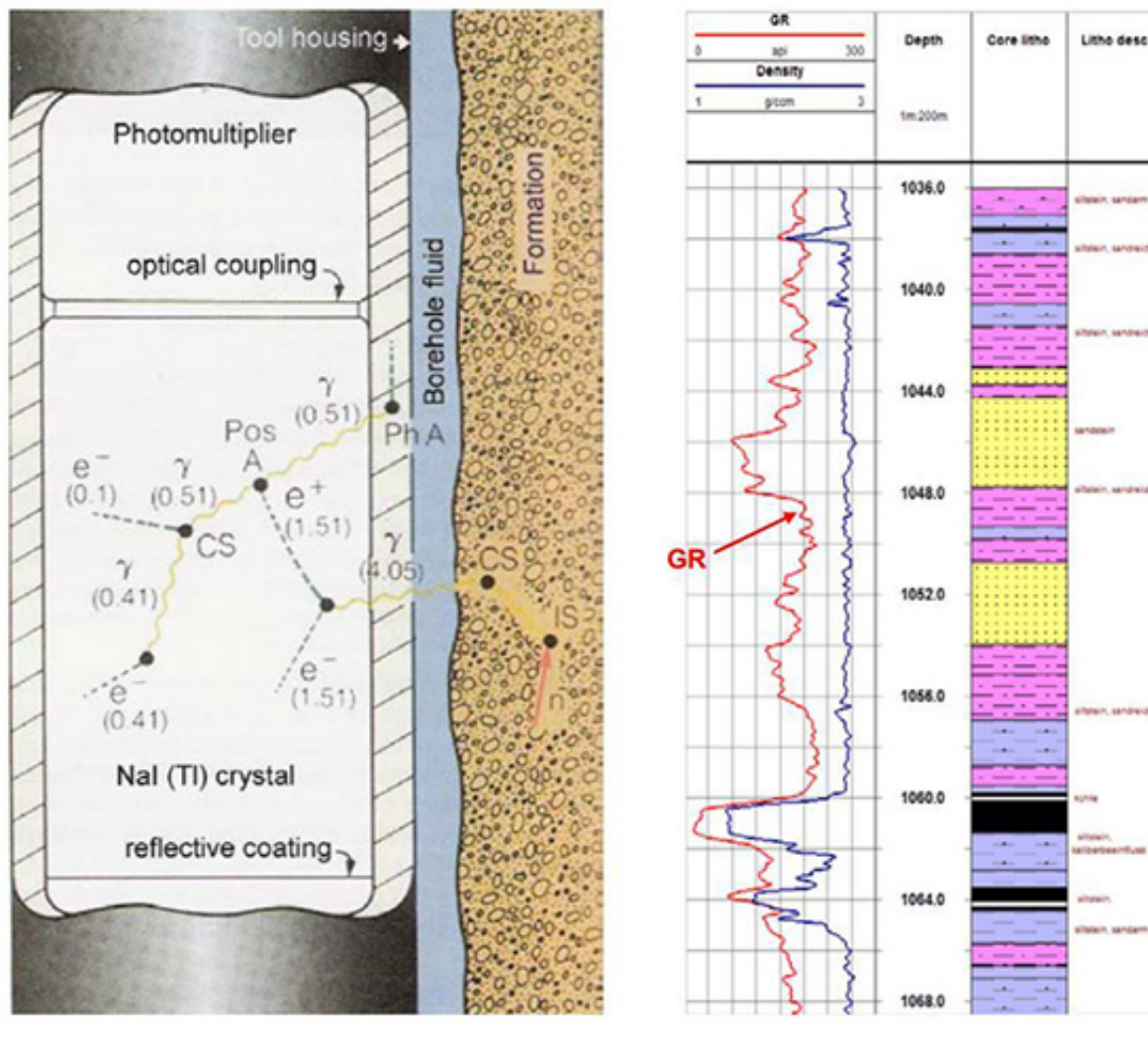
Measurement principle (left, O.&L. Serra, 2004) and typical GR responses and data display (right). Taken from the Q40GRA-1000 manual on the 23/06/2014.
