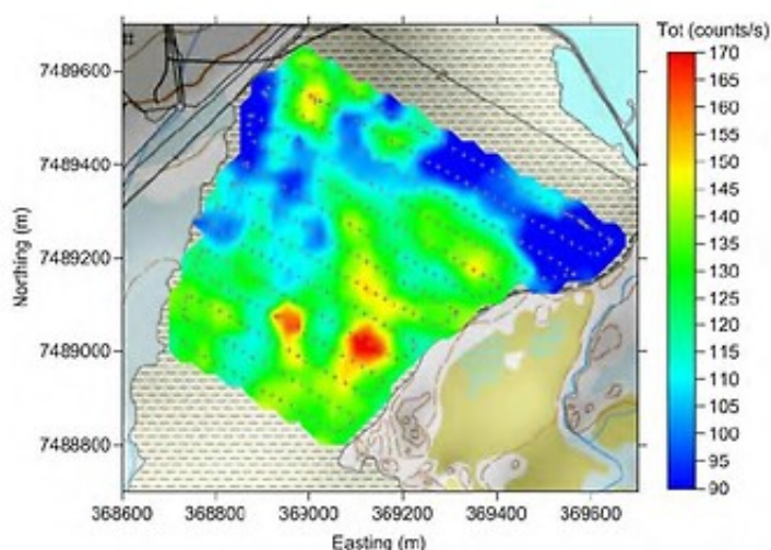
Contour Map of Total Intensity at 5m 1
