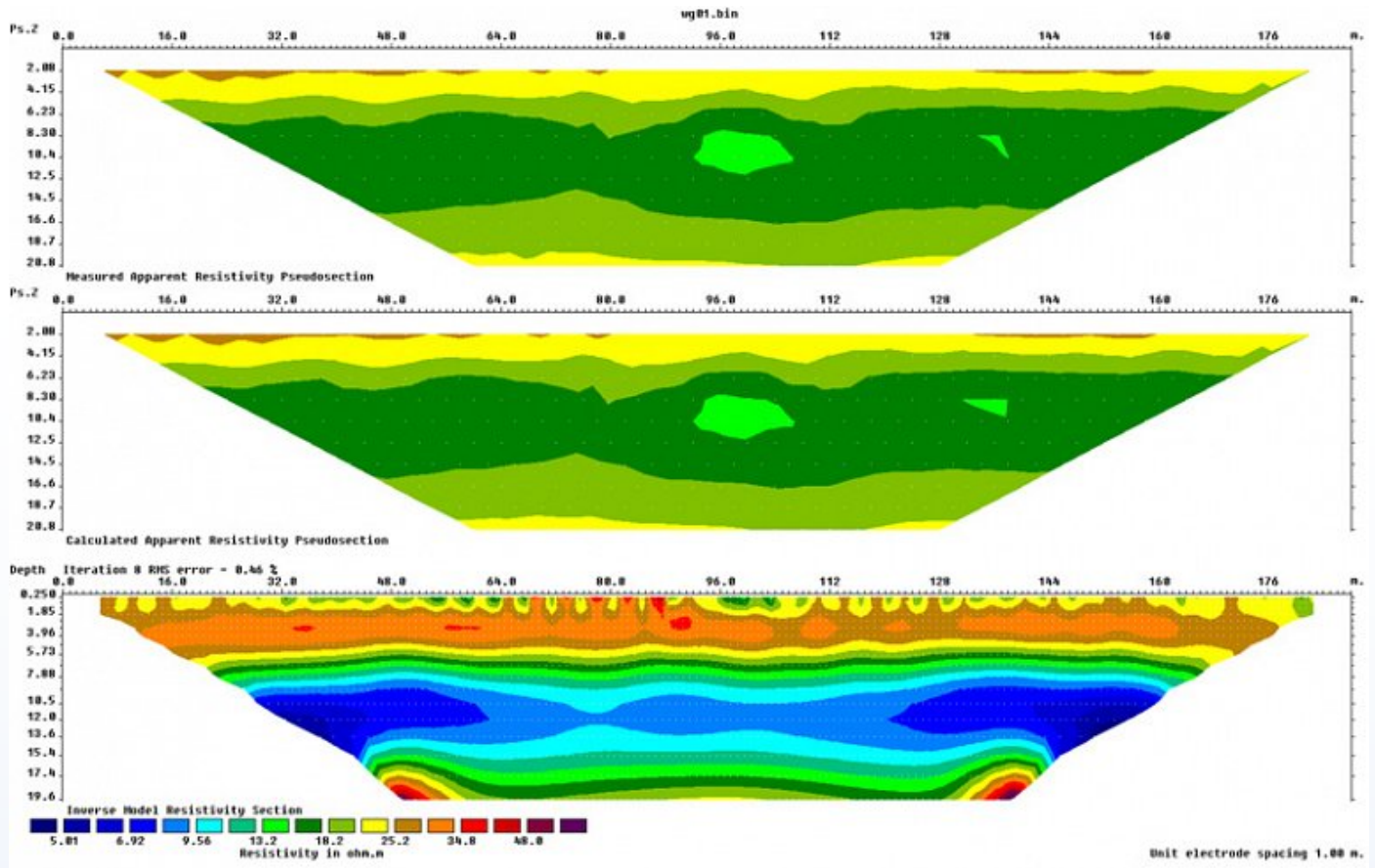
Resistivity model created using RES2DINV.
